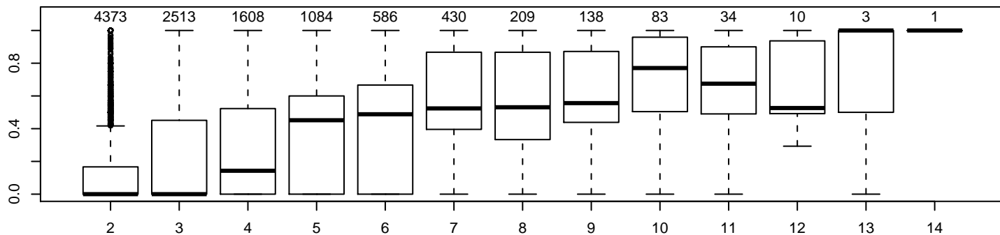
0 methylated CpG vs #CpGs
