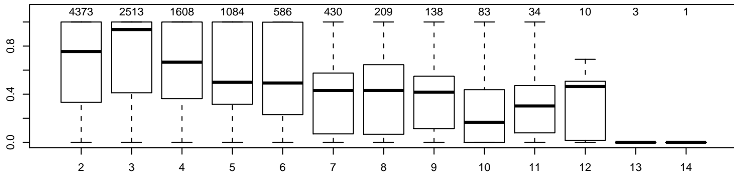
>1 methylated CpG vs #CpGs
