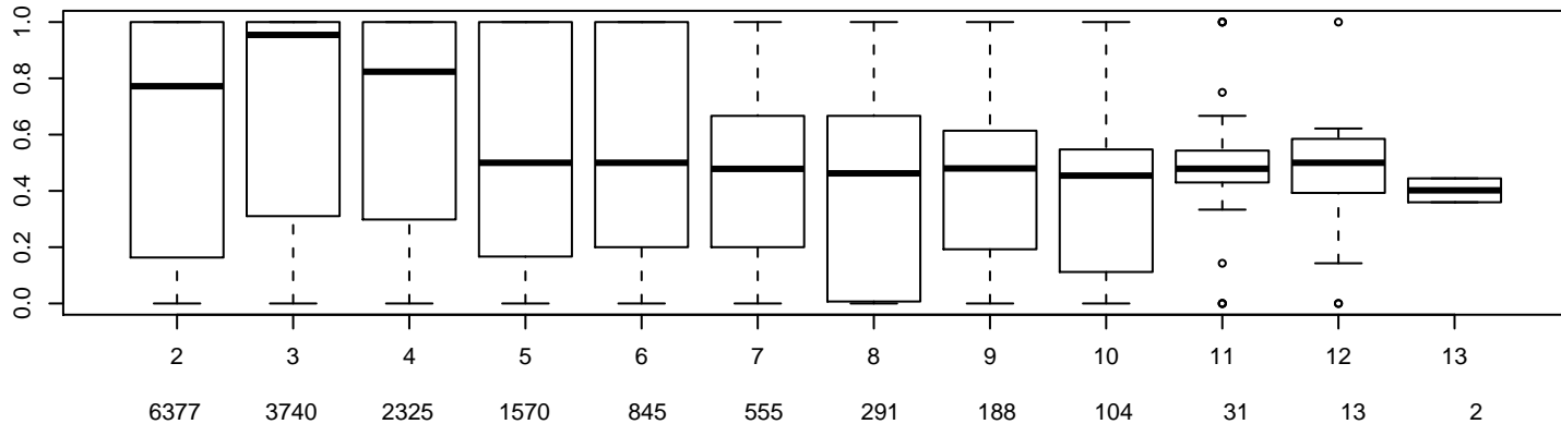
>1 methylated CpG vs #CpGs
