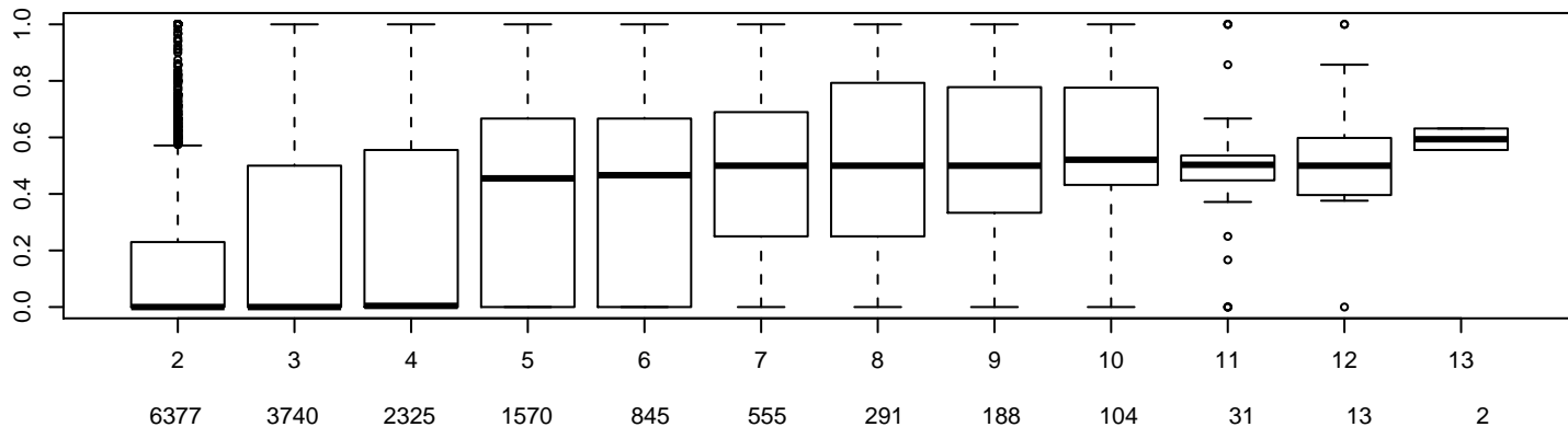
0 methylated CpG vs #CpGs
