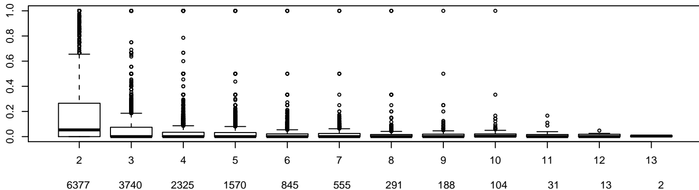
1 methylated CpG vs #CpGs
