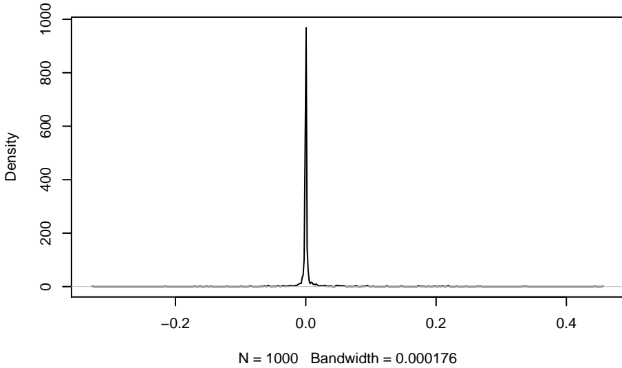
for SD= 0.2 overall fit, standartized back to a SD=1
