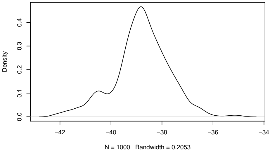
for SD= 0.05 overall fit, standartzed back to a SD=1
