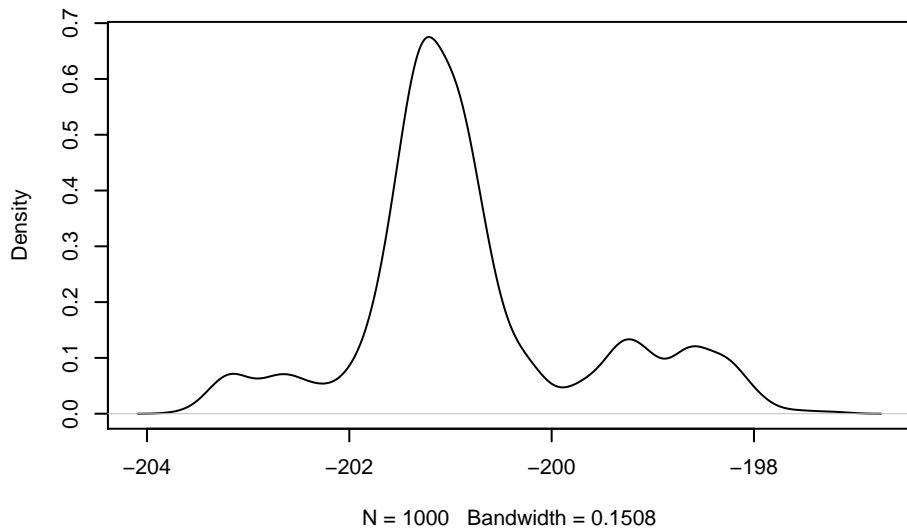
for SD= 0.01 overall fit, standartized back to a SD=1
