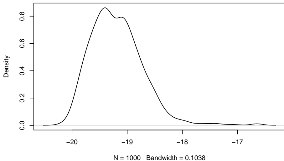
for SD= 0.1 overall fit, standartized back to a SD=1
