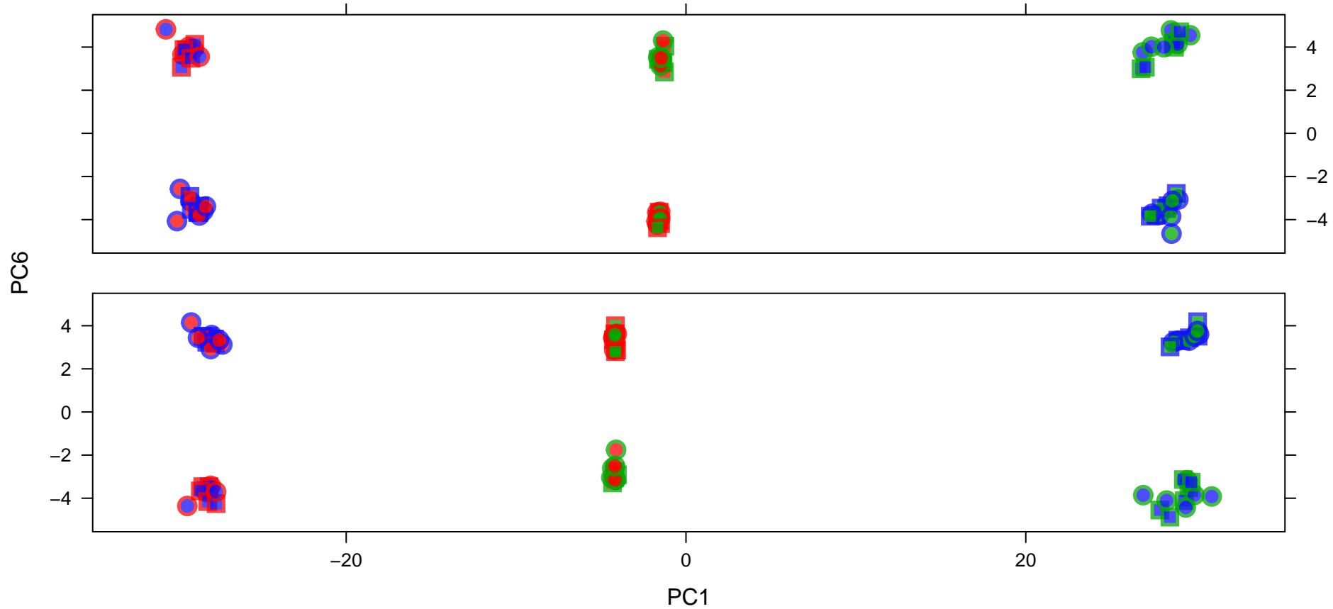
Autosomal allele-specific read count PC1 vs PC6
