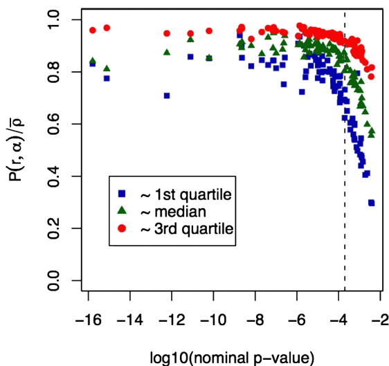
FIG. 2. Evaluation of the shortest distance approximation using 88 randomly selected gene expression traits. For each gene expression trait, the ratio P(r, \alpha) / \bar{p}(r) is plotted at three r 's, which are approximately the 1st quartile, median and 3rd quartile of P(r, \alpha) when P(r, \alpha) is between 0 and 1. The vertical broken line indicates the nominal p -value 2 \times 10^{-4} , which corresponds to genome-wide permutation p -value 0.05 \sim 0.10 .
